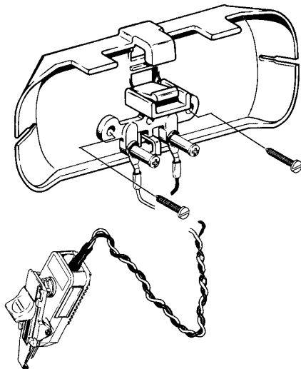
Figure 1 - 4047W Pair Test Plug Assembly
